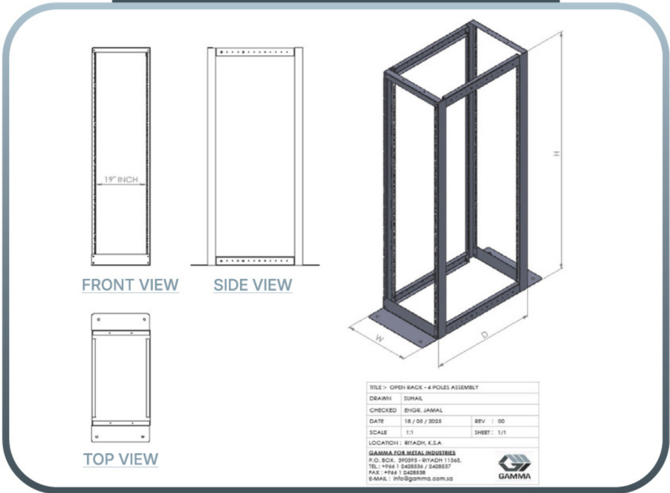
GAMMA OPEN RACK - 4 POLE - 19" INCH
