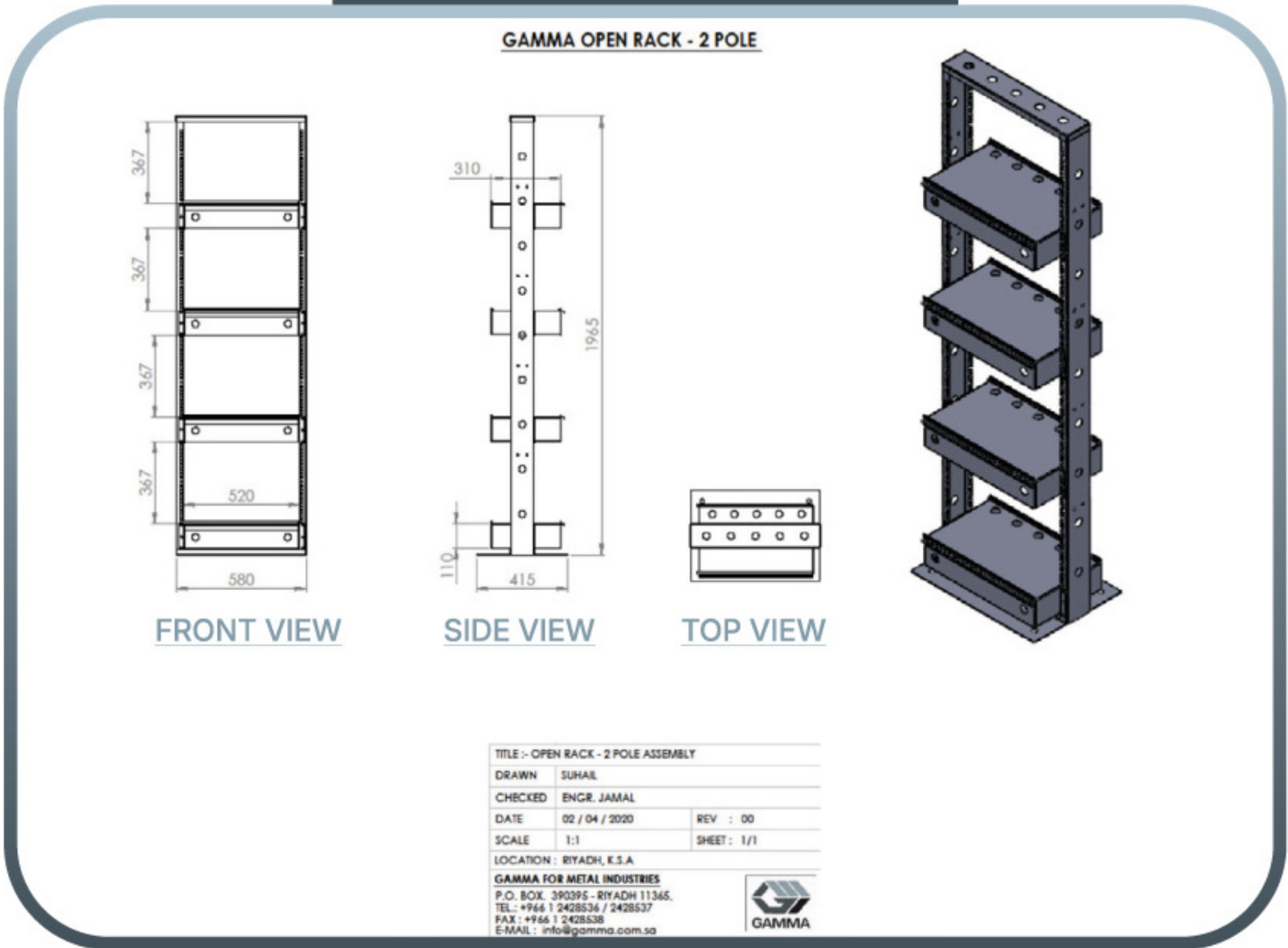
GAMMA OPEN RACK - 2 POLE
