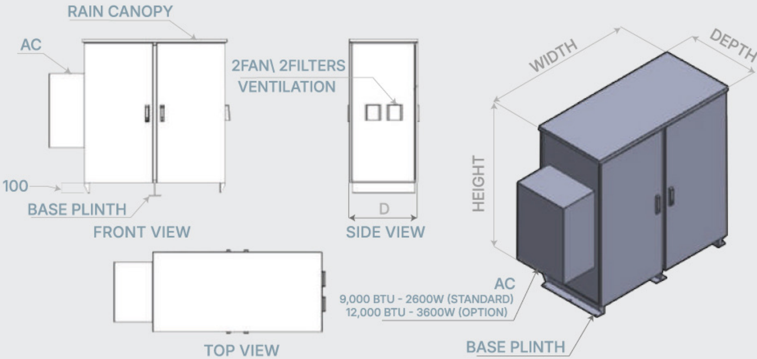
GAMMA OUTDOOR METAL ENCLOURES CABINETS WITH AC - IP66
