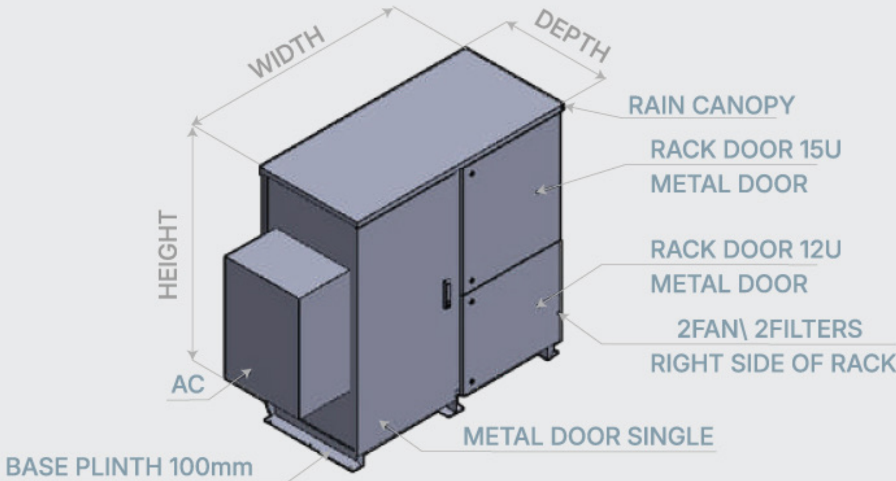
GAMMA OUTDOOR METAL ENCLOURES CABINETS
